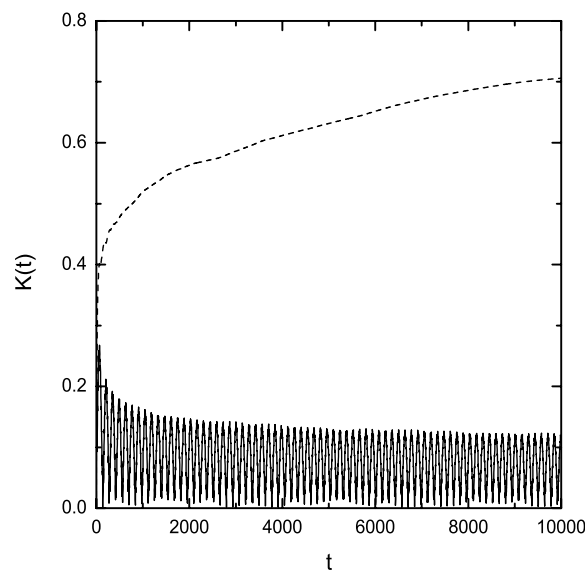
Figure 10. Application of the 0–1 test for the orbits of figure 1. K(t) oscillates with an amplitude decreasing towards K = 0 for the ordered orbit (solid line), while it tends to K = 1 for the chaotic orbit (dashed line).
