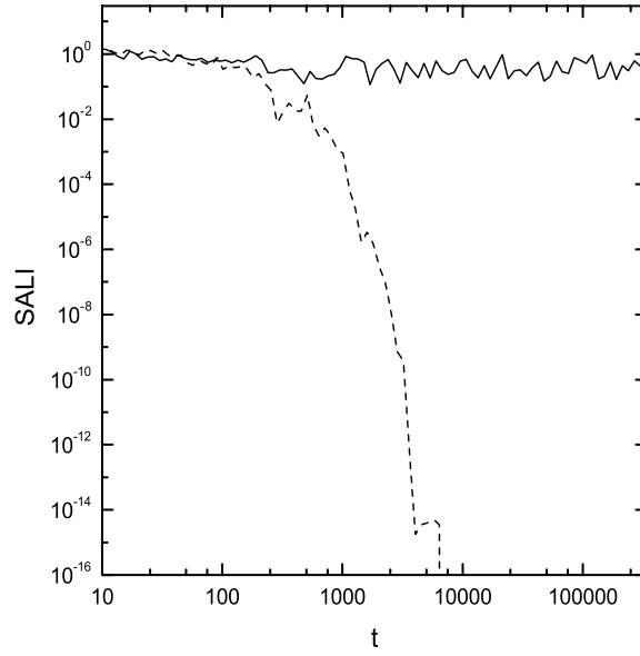
Figure 2. The time evolution of the SALI for an ordered (solid line) and a chaotic orbit (dashed line) of the 3D Hamiltonian (5), with initial conditions x = 0.010\,54 , y = 0.050\,60 , z = 0 , p_x = 0 , p_y = 0 , p_z \simeq 0.119\,06 and x = -0.073\,10 , y = 0 , z = 0 , p_x = 0.076\,95 , p_y = 0 , p_z \simeq 0.067\,60 , respectively.
